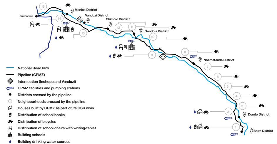
CPMZ pipeline route & sphere of influence
